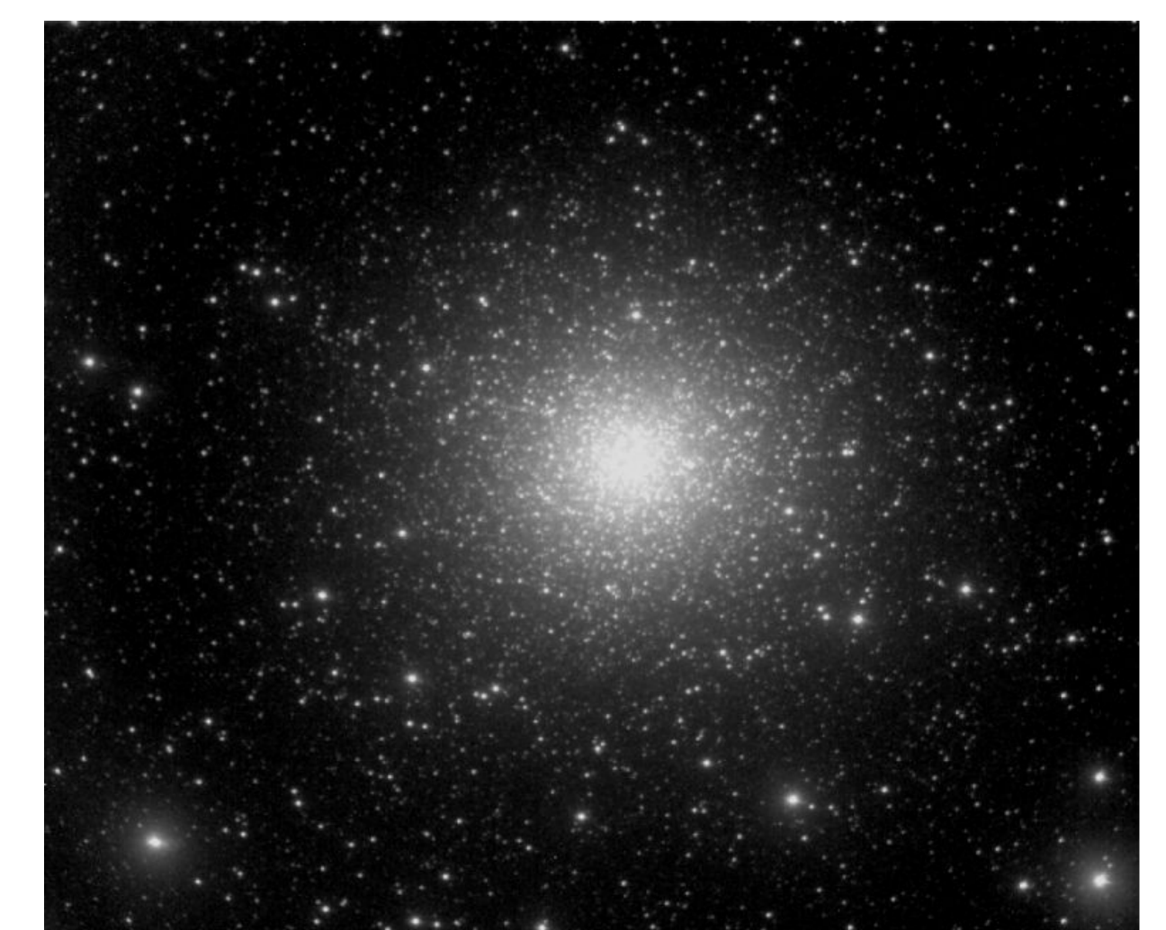
Figure 8: A 30 s exposure of Omega Centauri using 2 \times 2 pixel binning.
